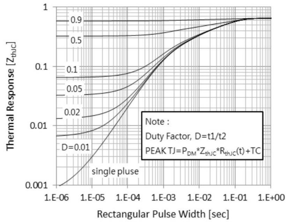
Figure 19. IGBT Transient Thermal Impedance
