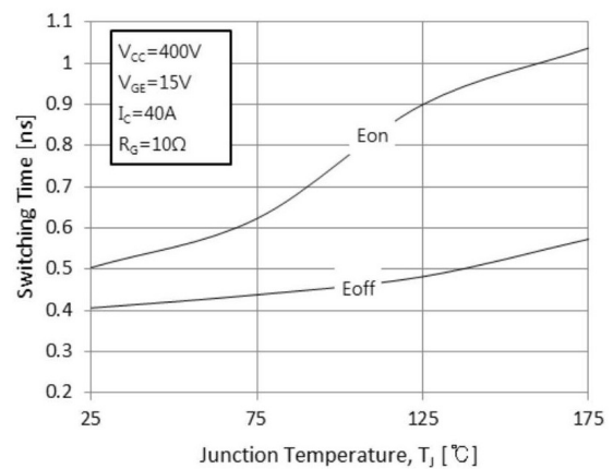
Figure 18. Switching Loss-Junction Temperature
