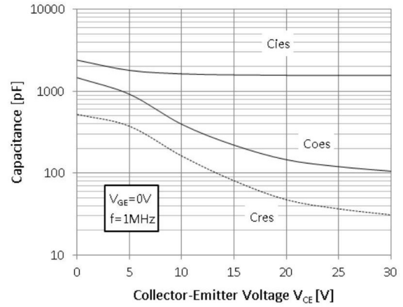
Figure 8. Typical Capacitance
