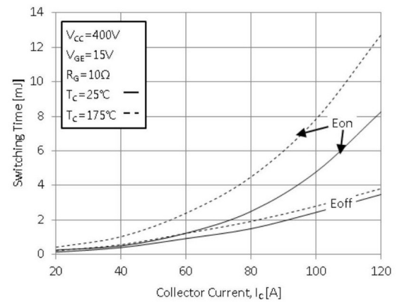
Figure 12. Switching Loss-Collector Current
