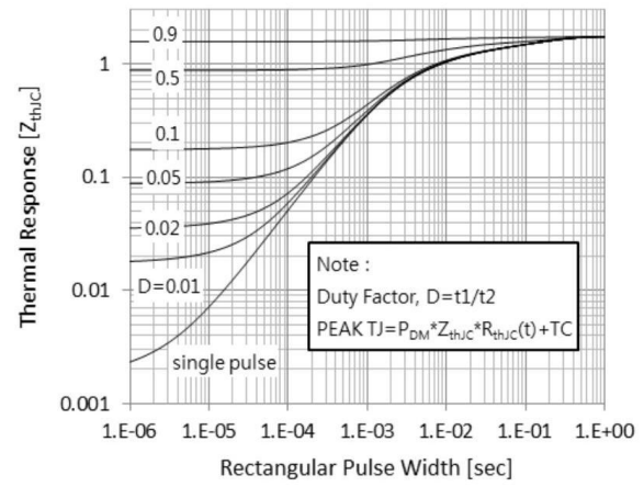
Figure 20. FRD Transient Thermal Impedance
