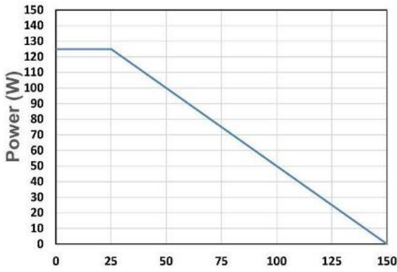
Figure 9. Power Dissipation
