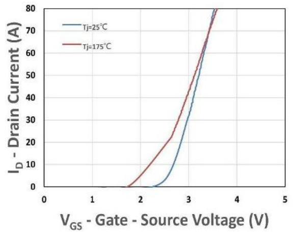
Figure 12. Transfer Characteristics
