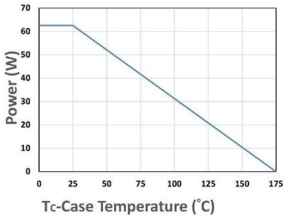
Figure 9. Power Dissipation
