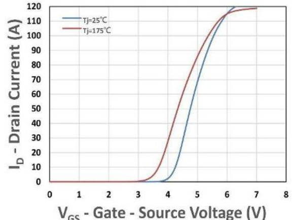
Figure 12. Transfer Characteristics
