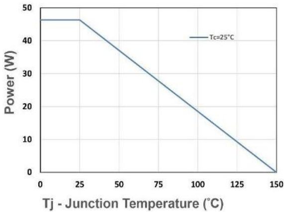
Figure 9. Power Dissipation
