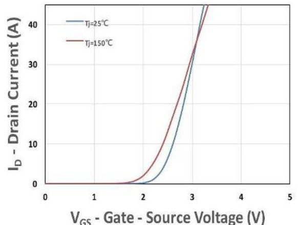
Figure 12. Transfer Characteristics
