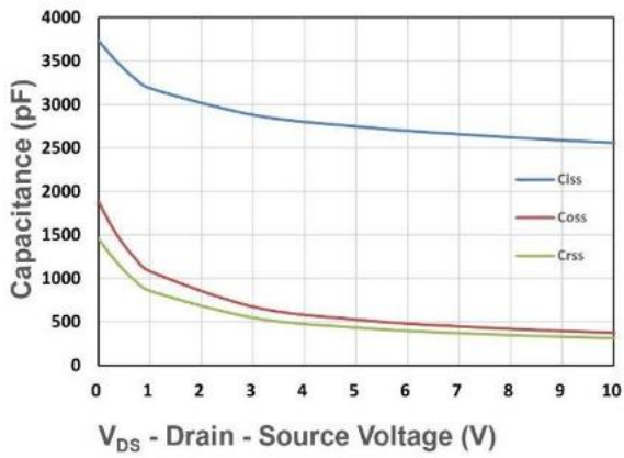
Figure 7. Capacitance
