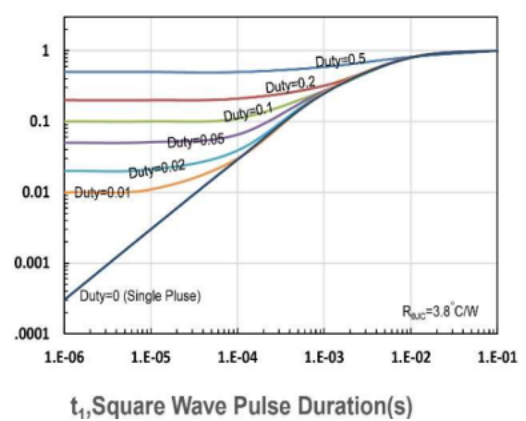
Figure 12. R_{\theta JC} Transient Thermal Impedance
