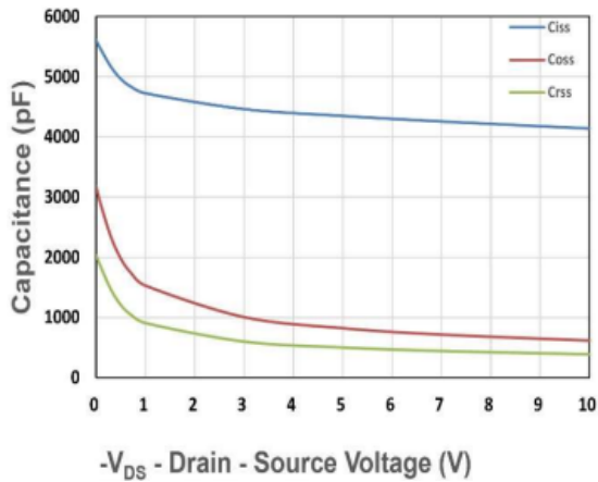
Figure 7. Capacitance
