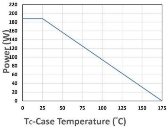
Figure 9. Power Dissipation
