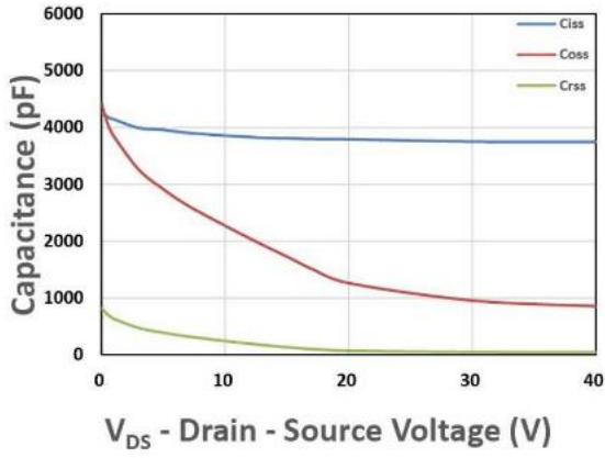
Figure 7. Capacitance
