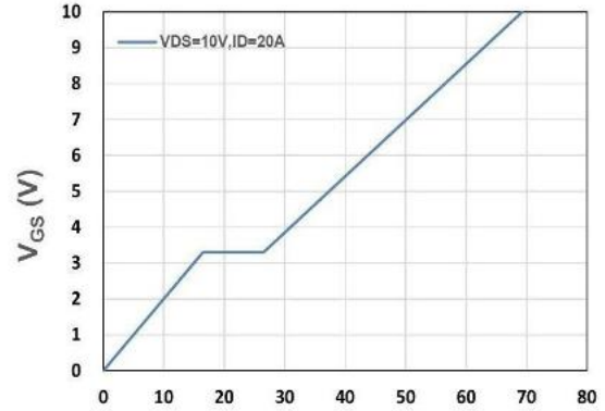
Q_g , Total Gate Charge (nC)
