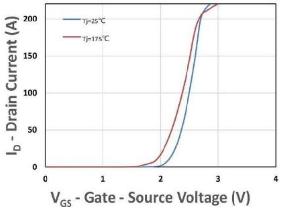
Figure 12. Transfer Characteristics
