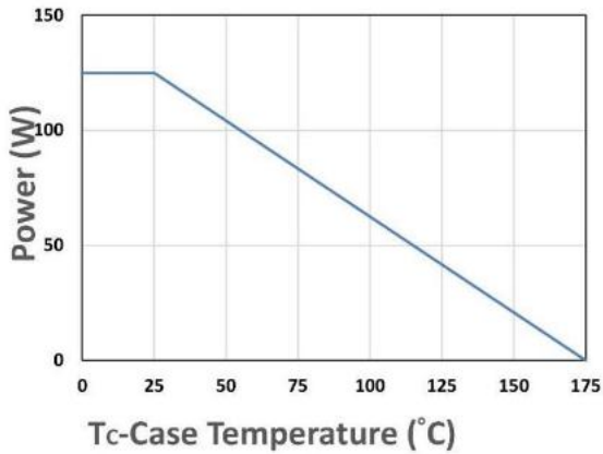
Figure 9. Power Dissipation
