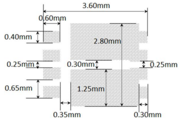
Suggested Pad Layout (Unit:mm)
