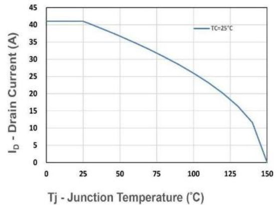
Figure 10. Drain Current
