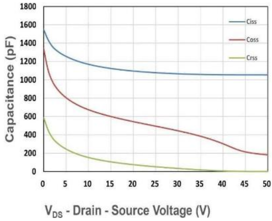
Figure 7. Capacitance
