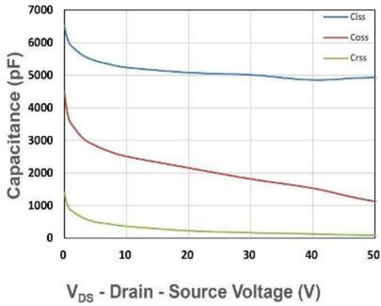
Figure 7. Capacitance
