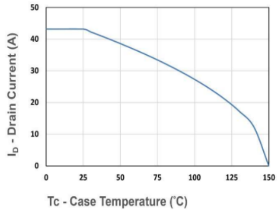
Figure 10. Drain Current
