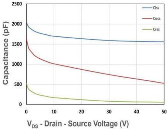
Figure 7. Capacitance
