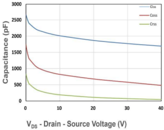
Figure 7. Capacitance
