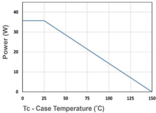
Figure 9. Power Dissipation
