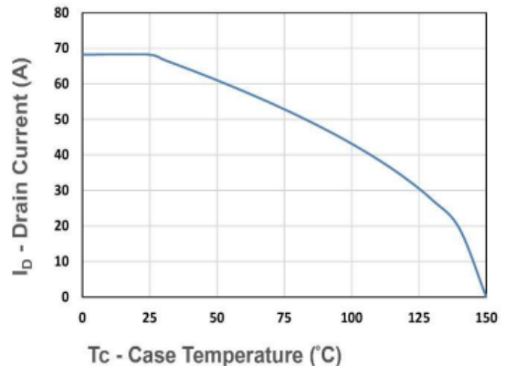
Figure 10. Drain Current
