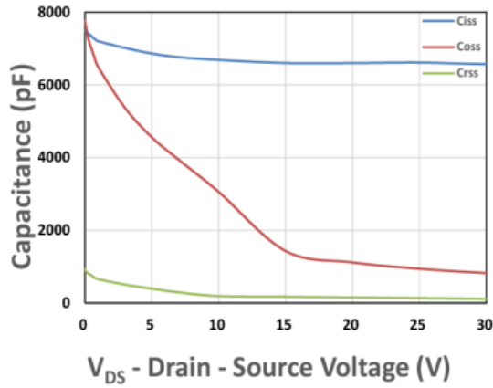
Figure 7. Capacitance
