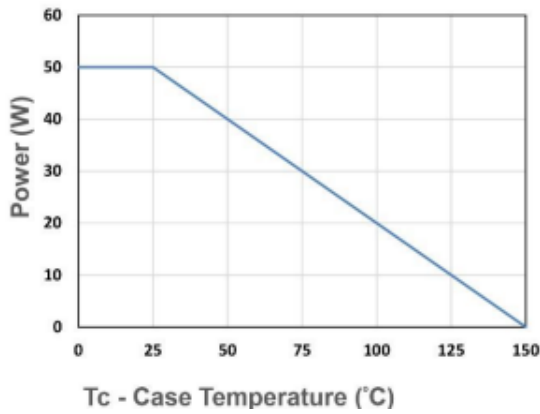
Figure 9. Power Dissipation
