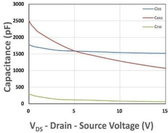
Figure 7. Capacitance
