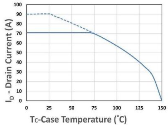
Figure 10. Drain Current
