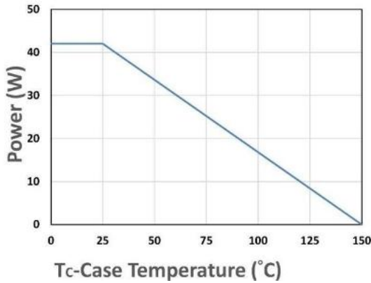
Figure 9. Power Dissipation
