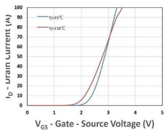
Figure 12. Transfer Characteristics
