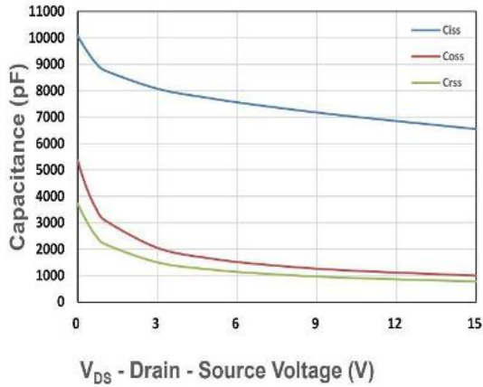
Figure 7. Capacitance
